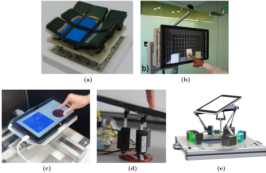
Figure 2.14 – Examples of actuated touchscreens. (a) Multi-faceted shape rendering with Tilt Displays [2]. (b) Normal force feedback from the TouchMover device [164]. (c) Planar force feedback system [174]. (d) Inclination rendering through linear actuators [83]. (e) Orientation display by the SurfTics system [51].
